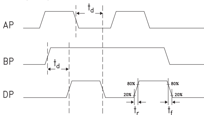
Timing Diagram
