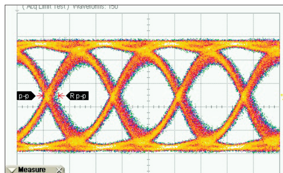
40 Gbps NRZ Differential Output Eye Diagram
